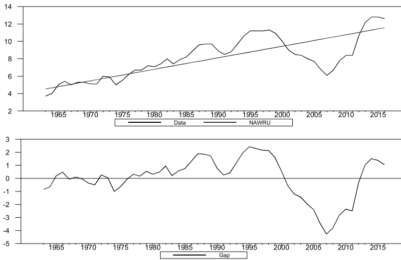
Figure 5.20: NAWRU with Local Trend
