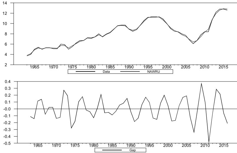
Figure 5.19: NAWRU with Damped Trend
