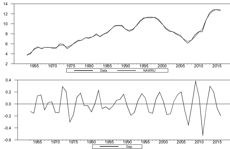
Figure 5.18: NAWRU with Damped Drift
