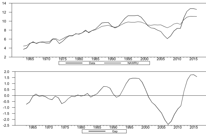
Figure 5.21: NAWRU with Damped Drift with Variance Restrictions
