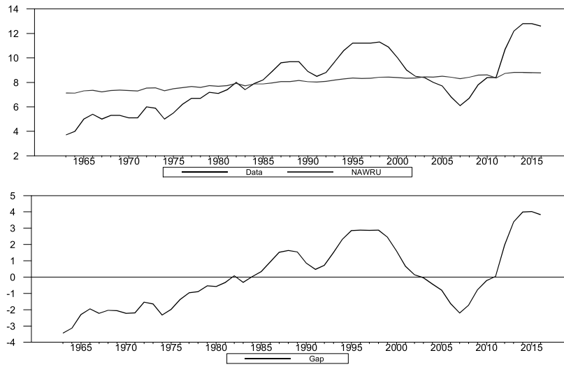
Figure 5.17: NAWRU with Local Level
