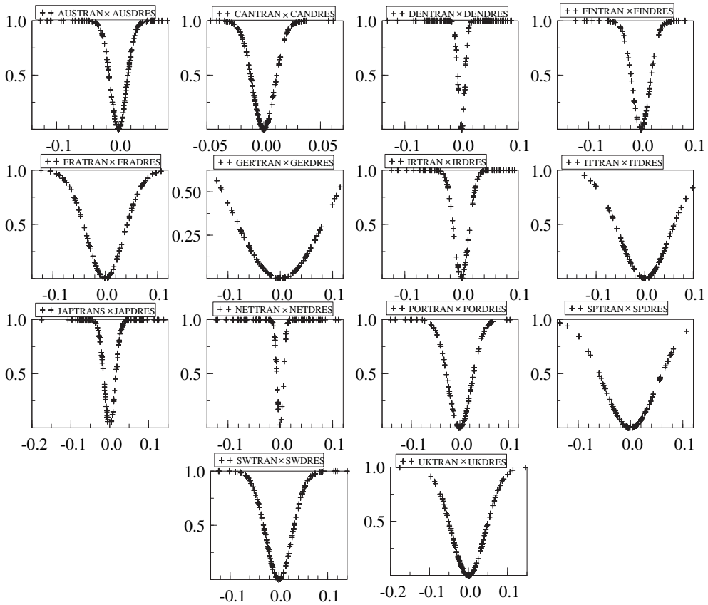
Fig. 3. Transition function vs. residuals F-Sup- t_{IN} test.
