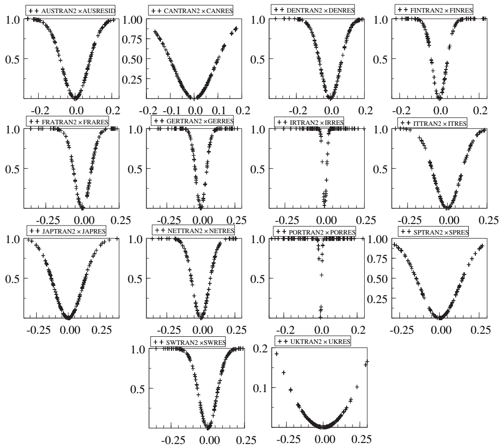
Fig. 4. Transition function vs. residuals F-t_{NL} test.
