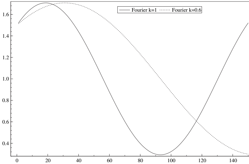
Fig. 1. Fourier functions with different frequencies.
