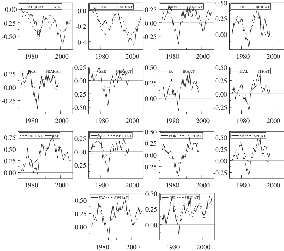
Fig. 2. RER and the Fourier Function.
